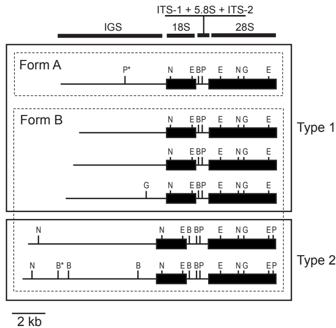
Figure 2.2. Restriction-site maps of ribosomal DNA repeat regions in North American Corbicula form A and form B. Restriction sites for a given enzyme are noted (P: Pvu II, N: Nco I, E: Eco RI, B: Bst EII, G: Bgl II). The diversity of array types in form B clams represents diversity within individual clams. IGS = intergenic spacer; ITS-1 = internal transcribed spacer 1; ITS-2 = internal transcribed spacer 2. The asterisk indicates a polymorphic restriction site (present in some copies of the array but not in others). These arrays are repeated in tandem in the genome, so hundreds of copies of each array are present in a given individual. Type 1 share restriction site patterns across 18S, ITS-1, 5.8S, ITS-2, and 28S, but differ in length and restriction pattern of IGS. Type 2 differs from Type 1 in the restriction pattern for 28S, the pattern and length of ITS-1 + 5.8S + ITS-2, and the pattern and length of the IGS.
